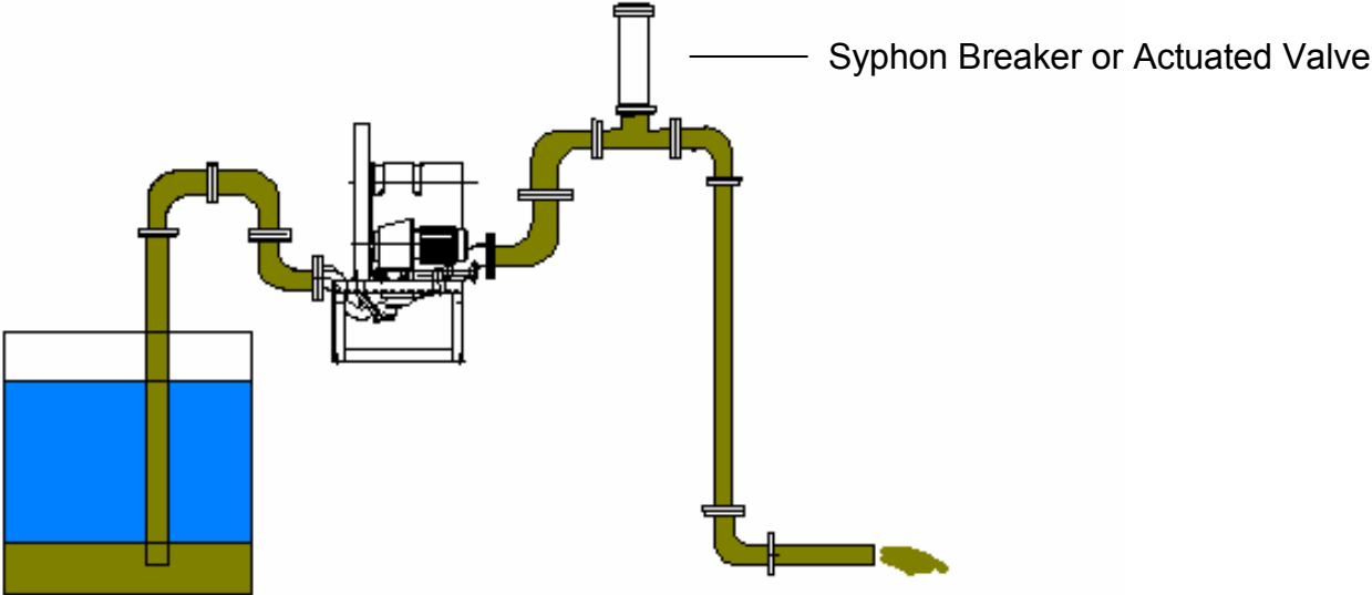
Fig 2 Suction Lift with Discharge to Gravity
