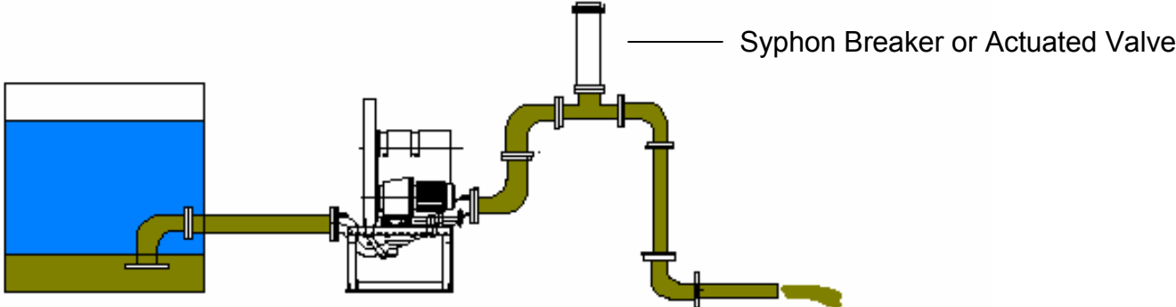
Fig 1 Positive Suction with Discharge to Gravity
