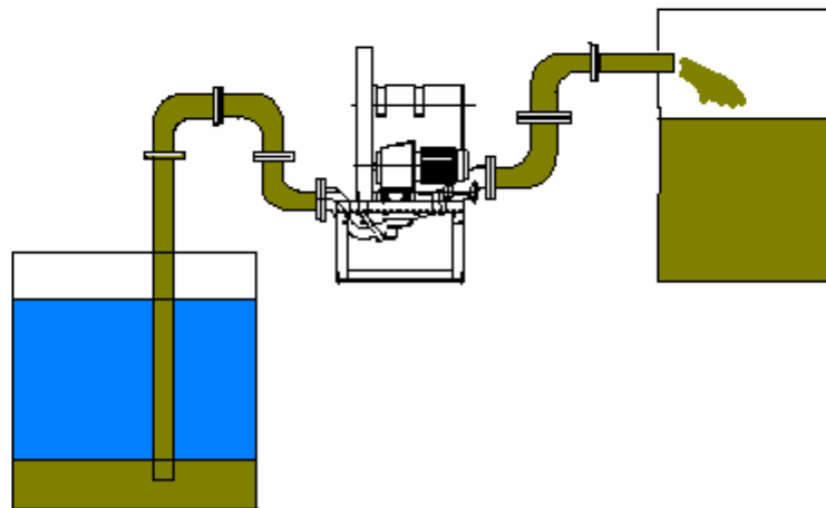
Fig 4 Suction Lift with Static Discharge Head
