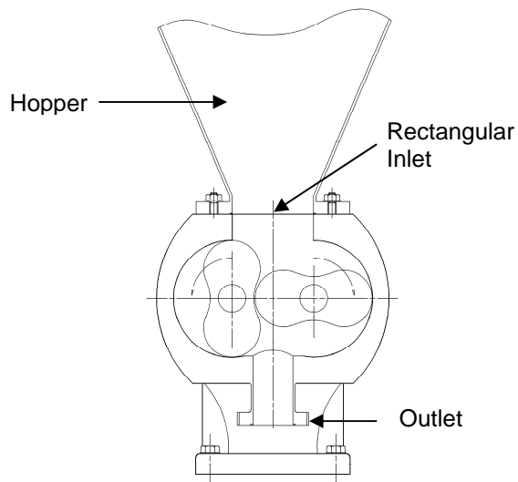
Typical Rectangular to Round Adaptor
